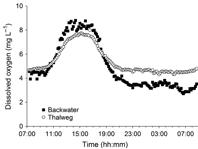
Fig. 2 O 2 concentrations in backwater 1 (closed squares) and the nearest thalweg (open circles).
