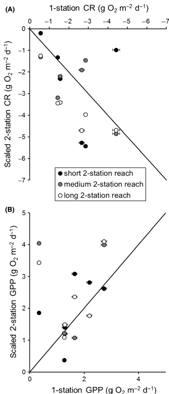
Fig. 4 One-station community respiration (CR) (A) and gross primary production (GPP) (B) rates compared to 2-station rates for short (black circles), medium (grey circles) and long (white circles) reaches. The black lines indicate 1:1 lines; thus, points occurring near the line indicate agreement between 1-station and 2-station rates. Error bars for 1-station estimates represent \pm 1 SD. For MSE, see Table 3.
