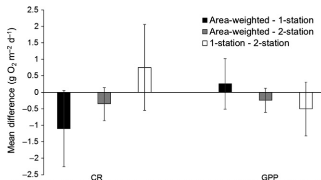
Fig. 5 Means and 95% confidence intervals for differences in community respiration (CR) and gross primary production (GPP) between methods after bootstrapping 5000 times. Black indicates differences between area-weighted and 1-station rates. Grey indicates differences between area-weighted and 2-station rates. White indicates differences between 1-station and 2-station rates.
