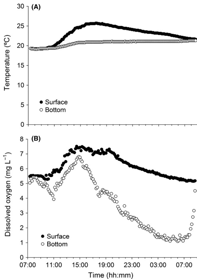
Fig. 3 Changes in temperature (A) and O 2 (B) between measurements made 15 cm below the surface (closed circles) and 15 cm above the bottom (open circles) of pool 3d. Pool 3b displayed similar patterns.
