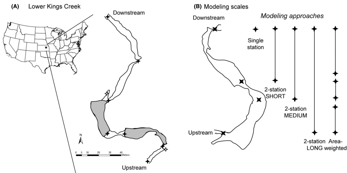
Fig. 1 (A) Konza Prairie Biological Station and locations of where O_2 probes were placed at site 3. Areas in white represent riffles and areas shaded in grey represent pools. Black stars indicate locations where O_2 probes were placed in the thalweg (the deepest area of the channel) and white stars represent locations where probes were placed in backwaters (where water flow was slower in side channels). (B) A conceptual model of how we categorised short, medium and long reaches and how we calculated metabolism using the area-weighted method.
